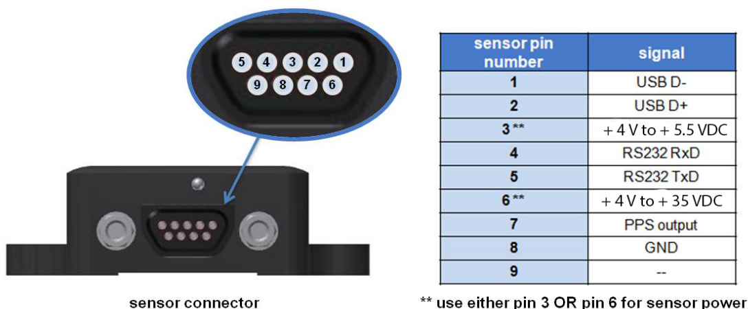
Figure 42 - Connector Wiring
