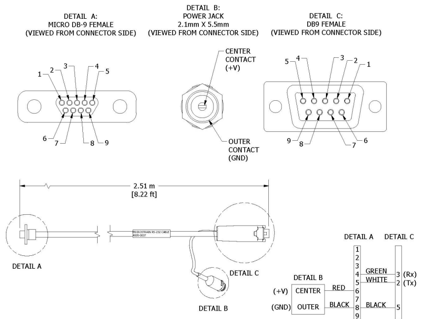
Figure 49 - Communications and power cable (RS232 Kits, PN: 4005-0037)
