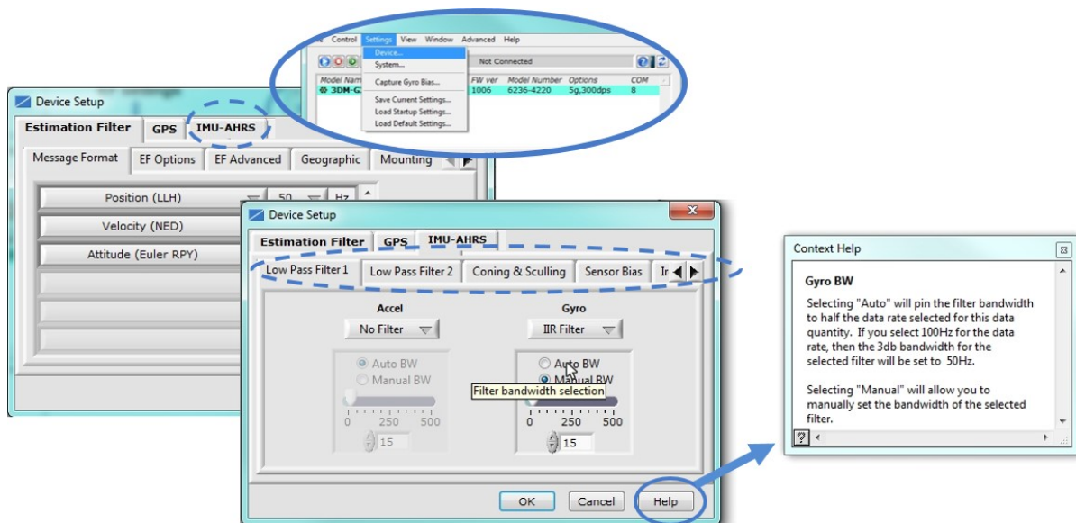
Figure 15 - IMU Settings
