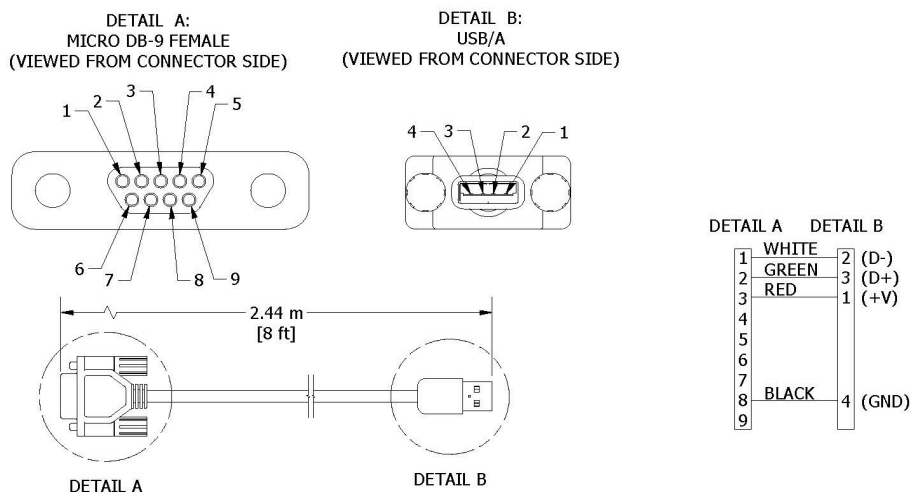
Figure 50 - Communications cable (USB Kits, PN: 9022-0019)
