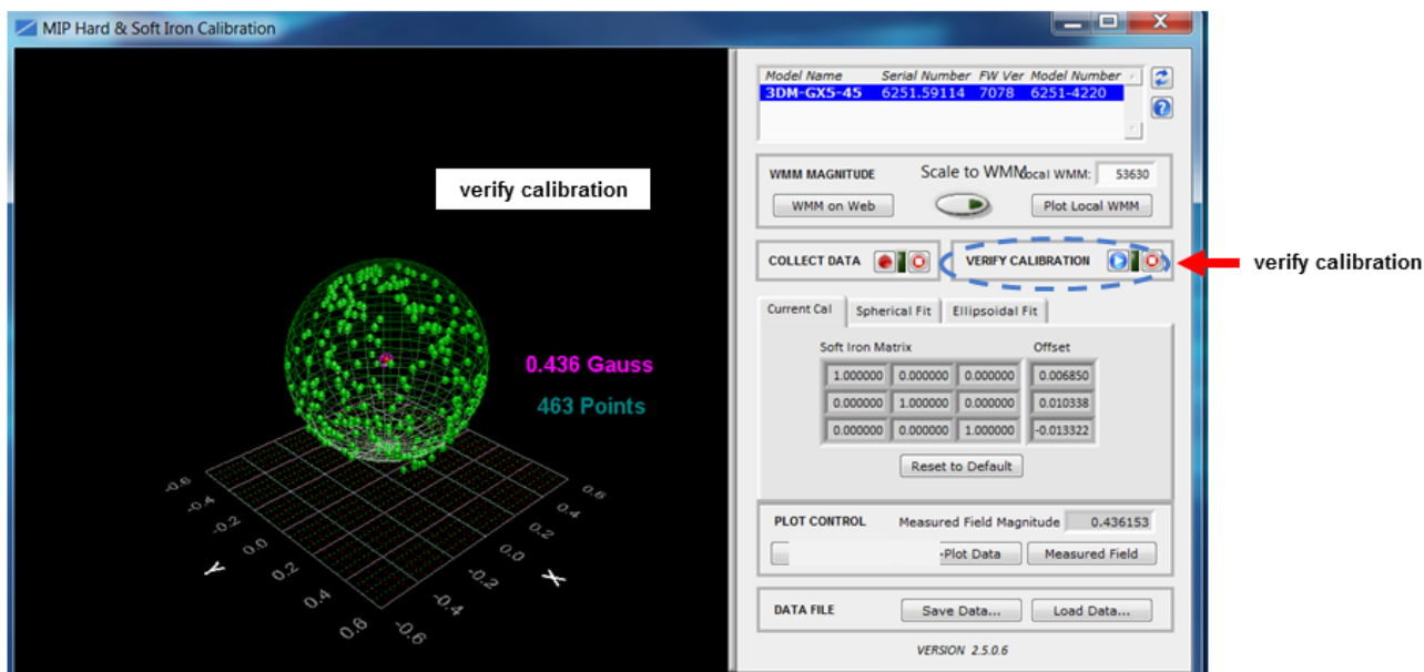
Figure 29 - Verify Calibration
