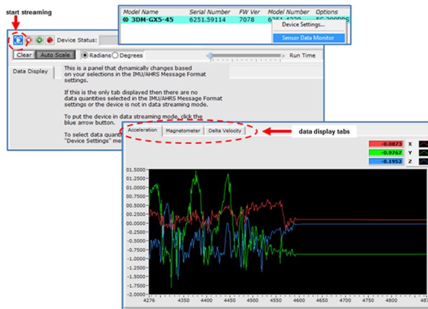
Figure 12 - Data Streaming
