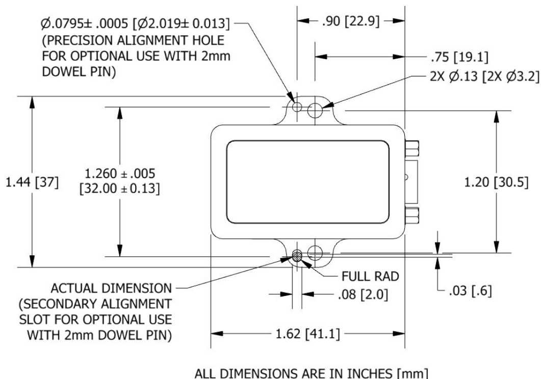
Figure 37 - Mounting the Sensor
