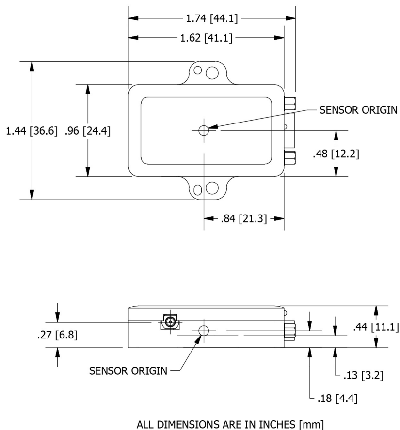
Figure 48 - 3DM-GX5-45 Sensor Origin
