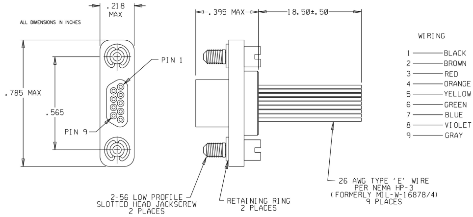
Figure 51 - Connector interface cable (sold separately, PN: 6224-0100)
