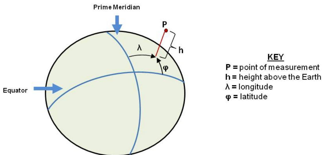
Figure 47 - World Geodetic System (WGS84) Reference Ellipsoid
